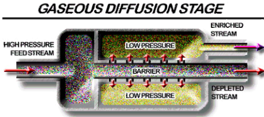
Figure 1: Schematic diagram of a single stage in a gaseous diffusion plant. The darker colors represent the UF_6 molecules that contain the heavier U-238 atoms, while the lighter colors represent gas molecules that contain the lighter U-235. After each stage the gas to the low pressure side of the barrier (i.e. the downstream side) has a slightly higher percentage of U-235 than the stage before. (Image courtesy of USEC Inc, http://www.usec.com/v2001_02/HTML/Aboutusec_enrichment.asp .)
